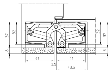
block frame
